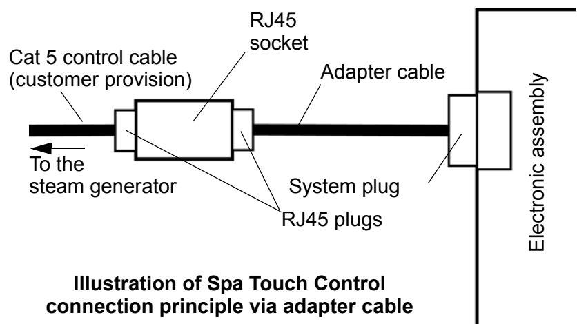
Adapter cable Cat 5 on system plug
